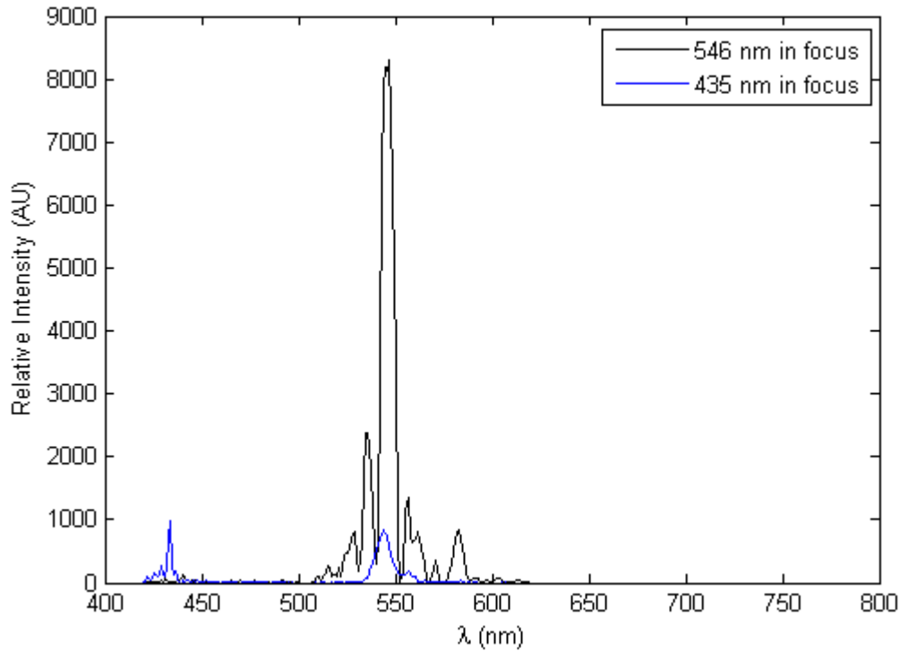
Figure 4.10: Spectrum of a Mercury lamp shining on a bar chart built with the gradient technique. It compares the spectra of 2 different CTE x data sets rather than comparing a CTE x measurement to an independent measurement. The black line is the spectrum with 546 nm in focus and the blue is when 435 nm was in focus. The smaller peaks near 546 nm were from artifacts of the bars that survived reconstruction.
