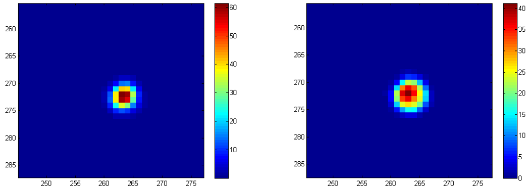
Figure 3.8: (L) The reconstructed image of the 641 nm emission from a Neon pen lamp within 1^\circ of the proper offset angle. (R) The reconstructed image of the 641 nm emission from a Neon pen lamp within 2^\circ of the proper offset angle . Selecting the proper angle to within 1^\circ tightened up the spot and increased the maximum intensity in the scene.
