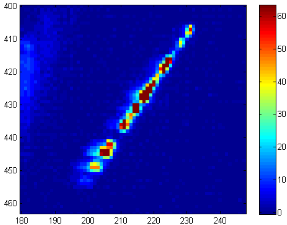
Figure 4.27: A zoomed in view of a raw frame from the Neon pen lamp behind a 25 \mu\text{m} pinhole. The shortest wavelengths are in the top right and the longest are bottom left. The almost continuous distribution of energy across the spectrum was why many lines peaks from the CTE x reconstruction in Figure 4.26 were not resolved.
